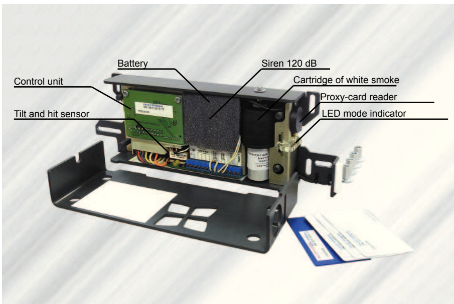
Elements of Faust-Terminal system
